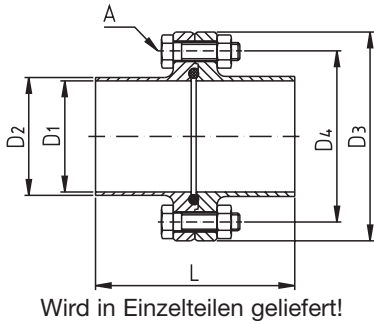
Flanschverbindung Zoll flange connection inch compl
