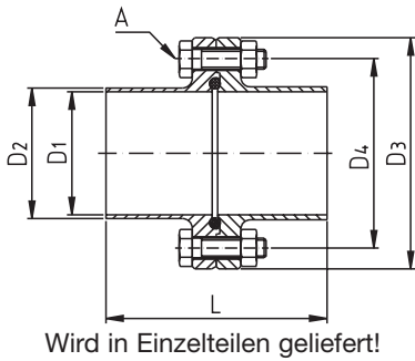
Flanschverbindung ISO flange connection compl
