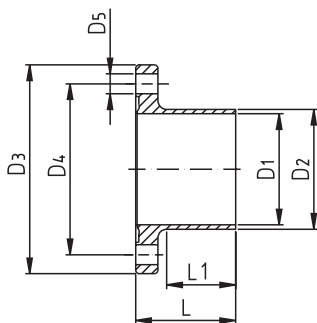
Bundflansch Zoll liner flange inch
